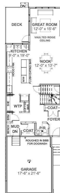
MAIN FLOOR PLAN 9'-1" CEILING HEIGHT
